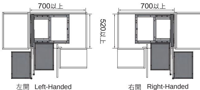
左開 Left-Handed
