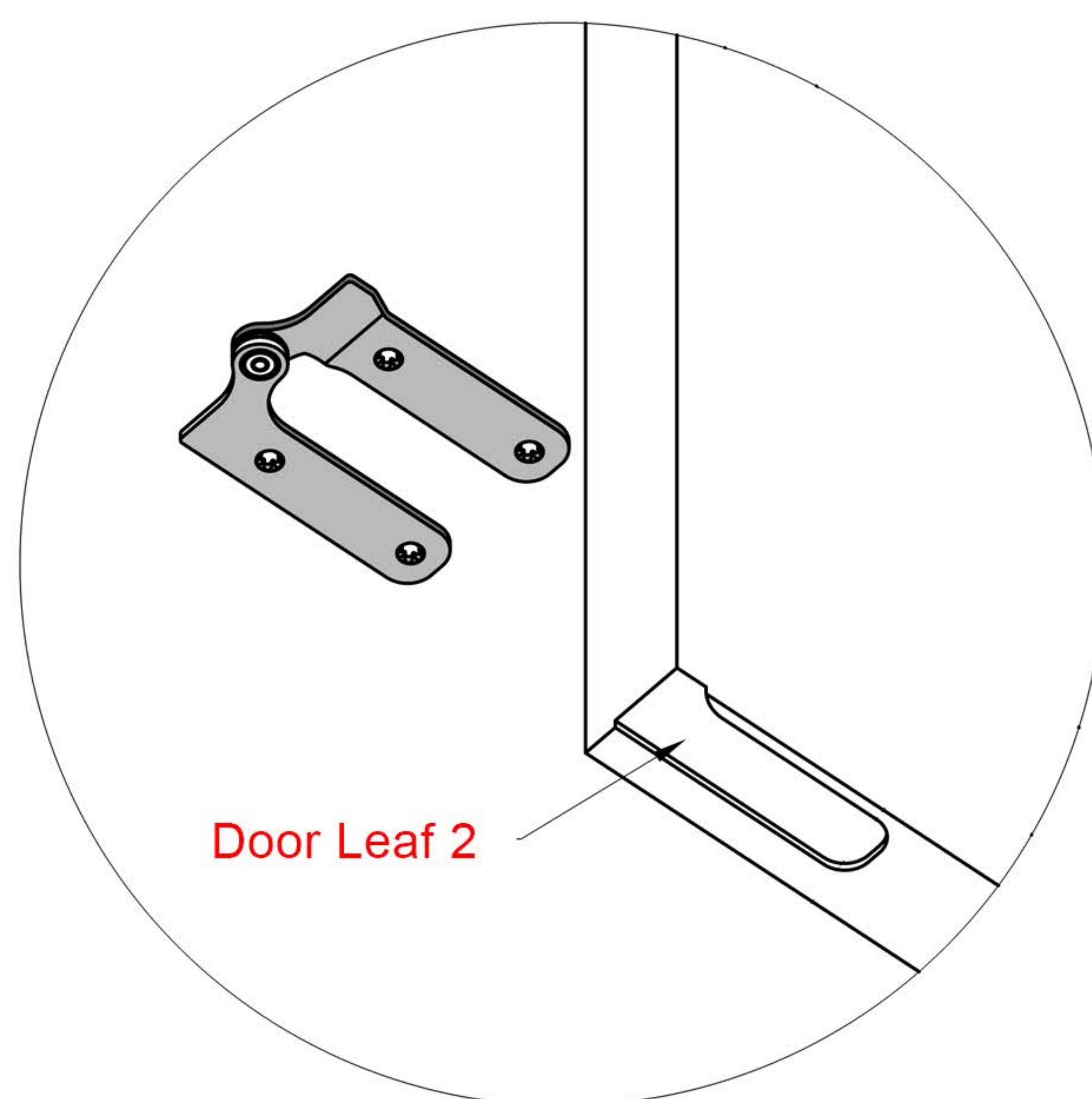
Detail D
