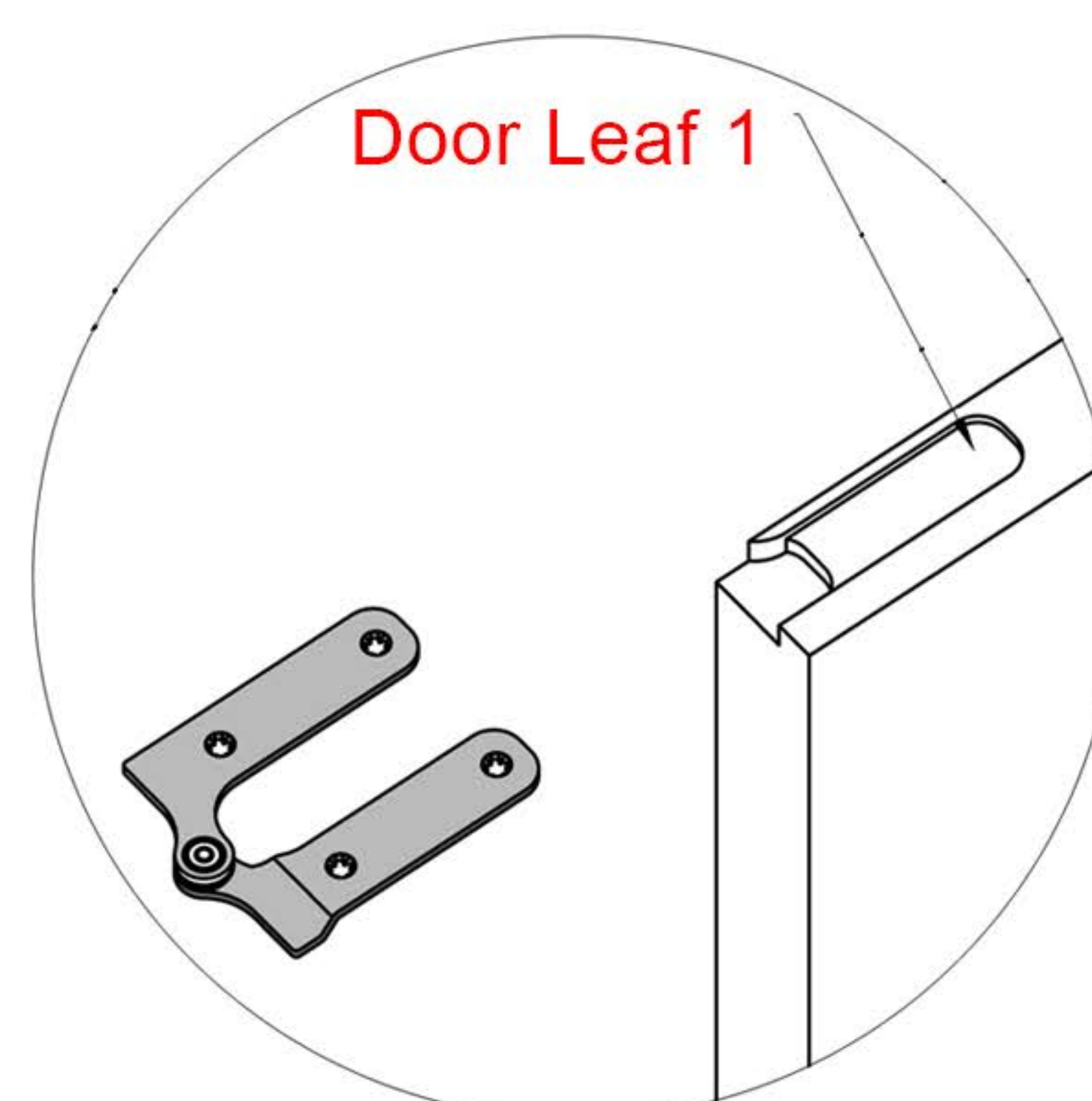
Detail C
